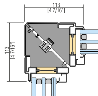
CORNER DETAIL
