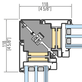
CORNER DETAIL
