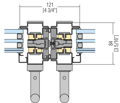
CENTRAL DETAIL
