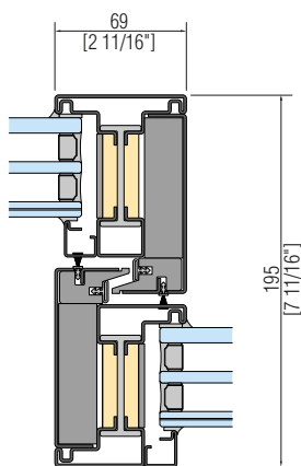
INTERLOCK DETAIL
