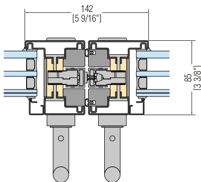
CENTRAL DETAIL
